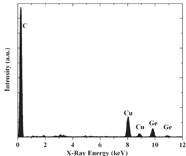
Fig. 4 EDS spectrum of Ge NCs dispersed on a carbon coated TEM copper grid.
